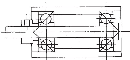
Solid Preload
